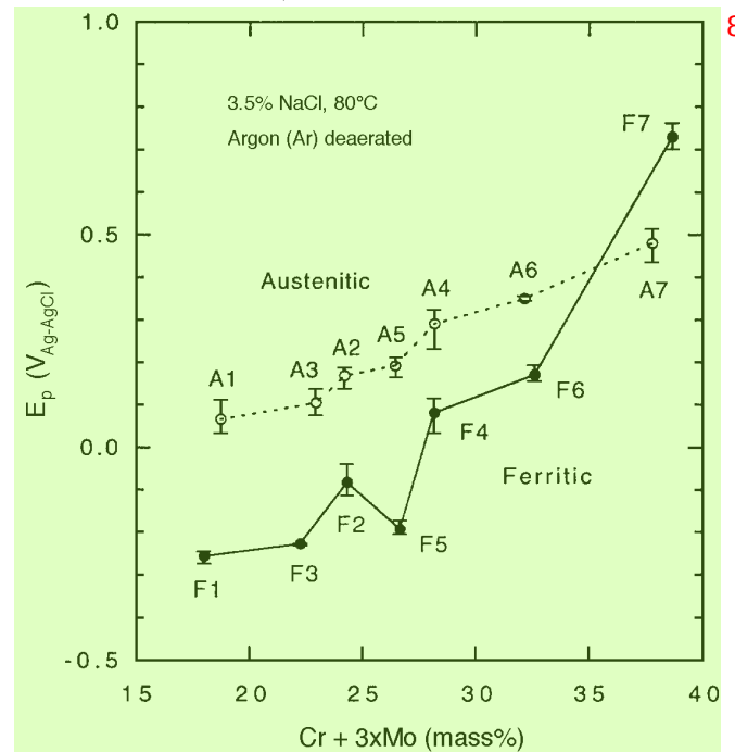
FIGURE 2. E p vs the Cr + 3xMo index for ferritic and austenitic SS in deaerated 3.5% NaCl solutions at 80°C.
