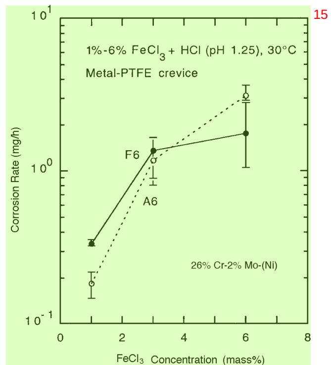
FIGURE 14. Crevice corrosion rate vs concentration of FeCl_3 for ferritic and austenitic SS containing 26% Cr and 2% Mo exposed to 1% to 6% FeCl_3 + HCl (pH 1.25) at 30°C.
